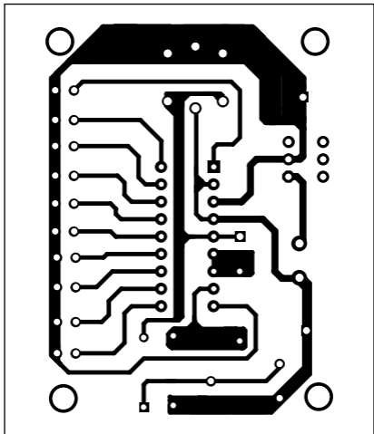
An actual-size, single-side PCB layout for the Remix BREATHLYZER2.0
