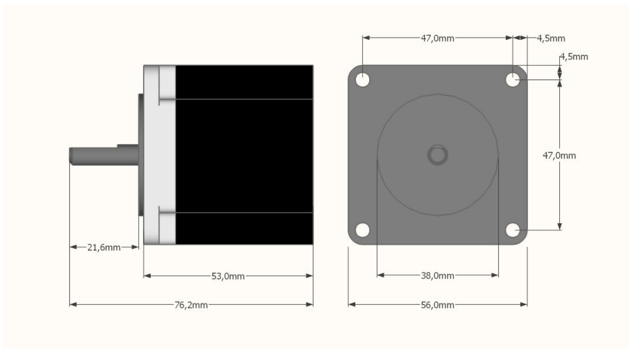
Motor Nema 23 (10Kgf)
