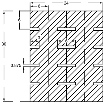
Horizontal Baseboards (x2)
