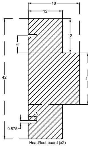
Head/foot board (x2)
