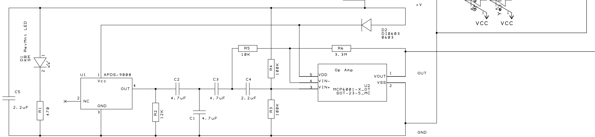
Optinote Circuit Schematic by Donovan Magryta 2018
