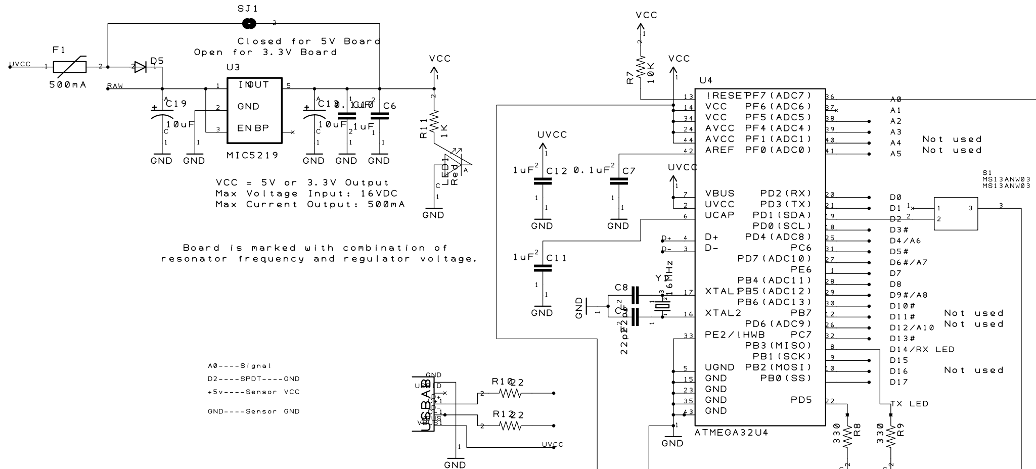
Optinote Circuit Schematic by Donovan Magryta 2018
