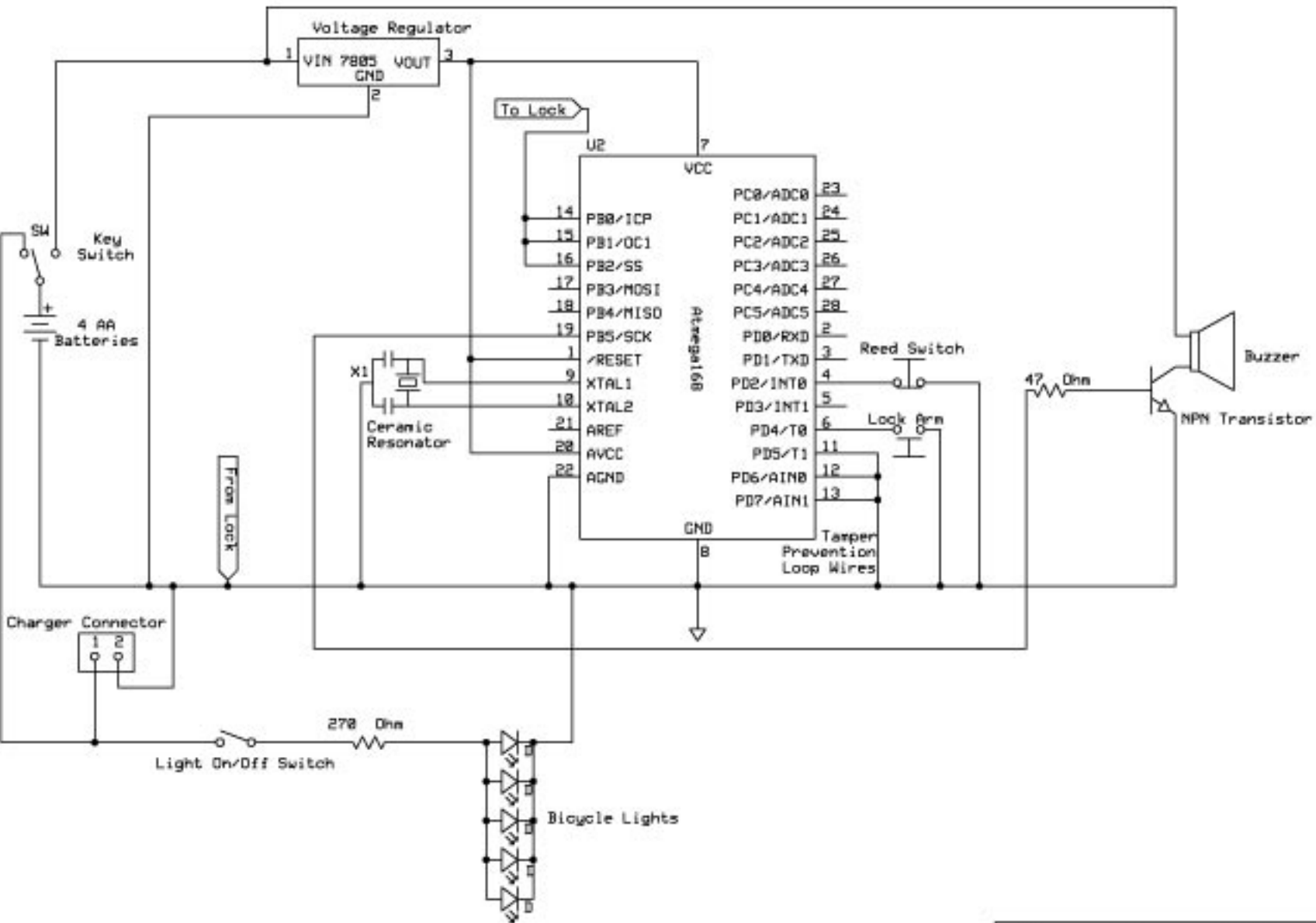
Standaloneduino Bike Alarm Circuit Schematic Rev 1.8 11/19/2008 Page 1 of 1
