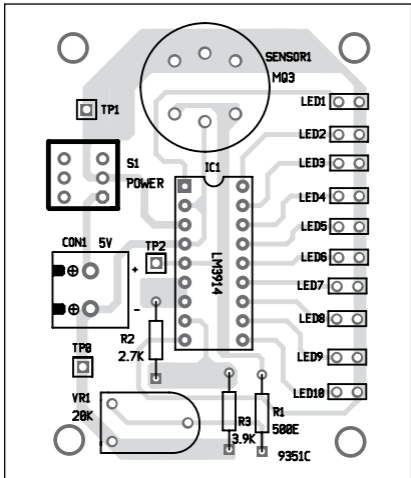
Component layout for the PCB
